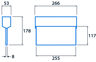
Ceiling Mounting
